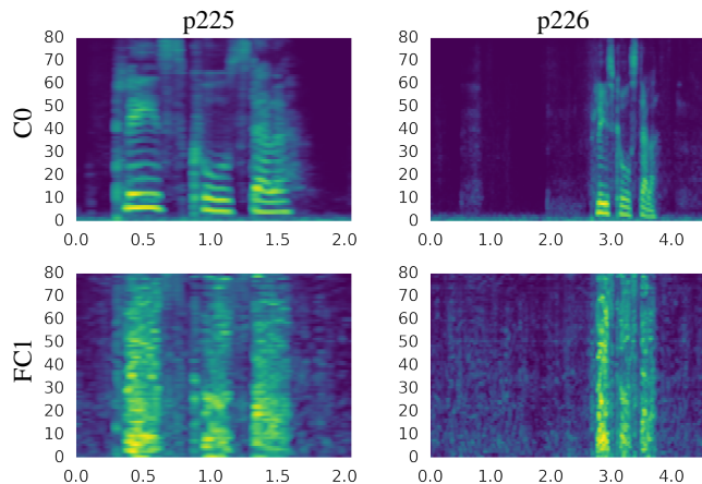
Fig. 1. Mel spectrograms of waveforms reconstructed from layers C0 and FC1 of speakers p225 (female) and p226 (male) from the VCTK dataset. The reconstructions from C0 are nearly exact, while the reconstructions from FC1 are very noisy and are barely intelligible.
