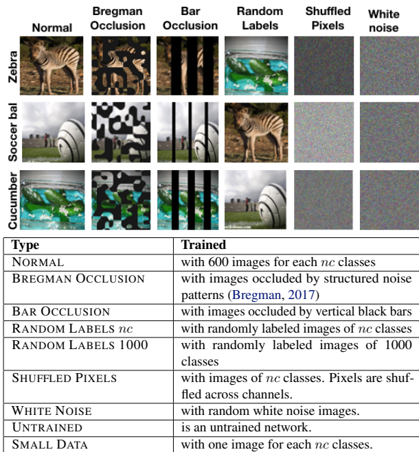
Figure 4. Descriptions of running conditions and a subset of training data used to test hypotheses
