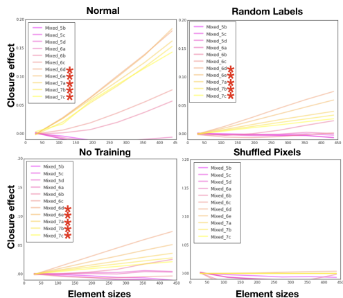
Figure 6. H1. Inception Results closely mirror simple network results (Fig. 5)
