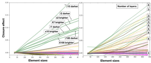
Figure 9. H4.,H5. The closure effect does not have clear pattern of change as images become brighter/darker or as the depth of network and/or number of classes trained change. (significance omitted for simplicity)
