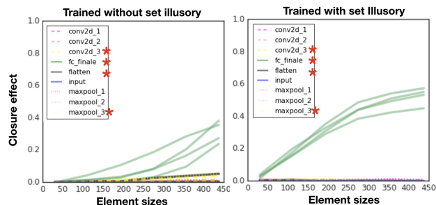
Figure 3. Sanity check experiment: Networks trained with set I have more closure effect. Multiple lines represent multiple runs of the same condition.
