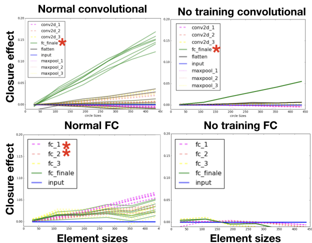
Figure 10. H7. Having convolutional layers correlates with stronger closure effect, in UNTRAINED and NORMAL networks. Note that accuracy of FC is much lower than convolutional network. Layers resulted in significance are marked with *.
