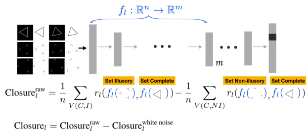
Figure 1. The experiment framework for measuring closure effect in NN
