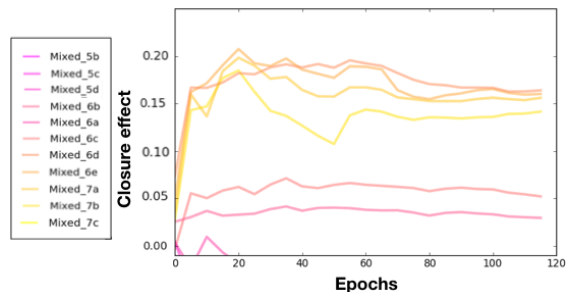
Figure 8. H3. The closure effect in the last layer reaches its peak earlier in the training process, then decreases somewhat as it converges. Other layers seem to continue to fluctuate before converging. For degenerated networks, the effect is quickly forgotten. Showing results from Inception.
