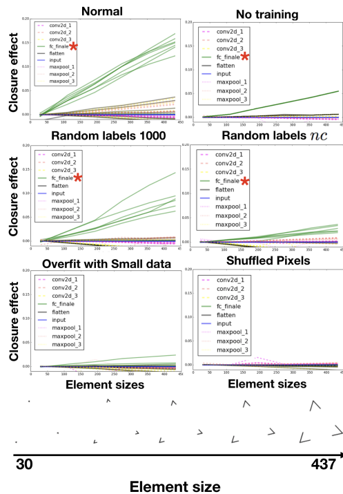
Figure 5. H1. Each graphs shows the closure effect as element size increases for each layer for each running condition. Multiple lines represent multiple runs for the same condition. Note that input (blue line) stays very small as we control the pixel overlap. Layers that resulted in statistical significance are marked with red *.
