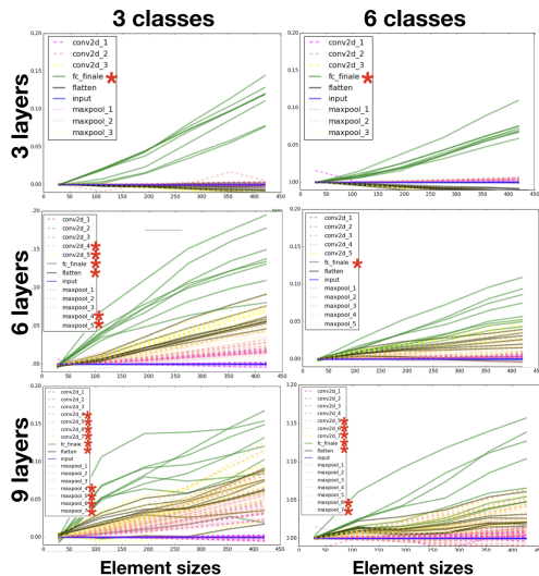
Figure 7. H2. Layers close to the prediction layer typically exhibit stronger closure effect. Layers resulted in significance in Welch t -test are marked with *.
