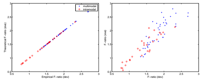
(a) Empirical F-ratio vs. theoretical F-ratio
