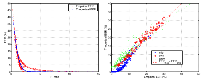
(a) Empirical and theoretical EER vs. F-ratio
