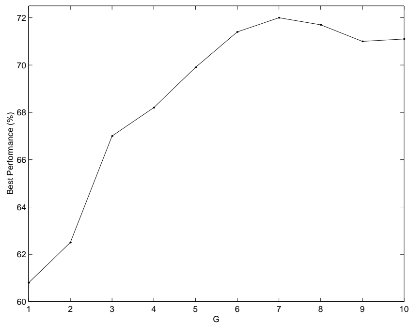
Figure 2: Best Performance of the WI systems as a function of G . For each value of G , the best performance obtained among the systems with 10 \leq S \leq 20 is plotted. G is increased until it is not possible to obtain any more improvement of the performance.
