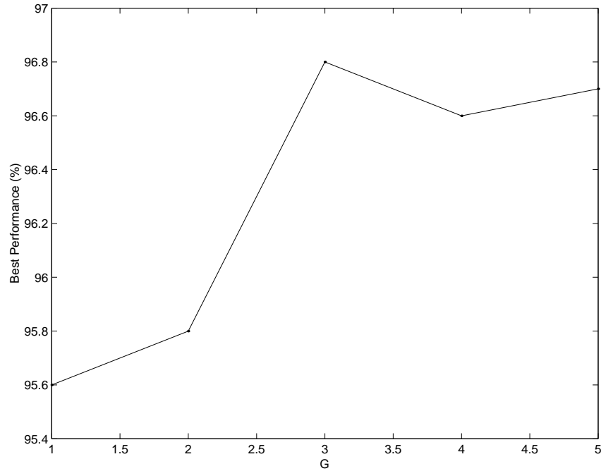
Figure 3: Performance of the WD systems as a function of G . For each value of G , the best performance obtained among the systems with 6 \leq S \leq 16 is plotted. G is increased until it is not possible to obtain any more improvement of the performance.
