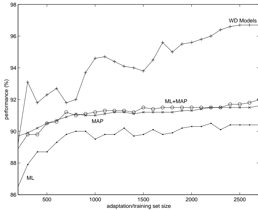
Figure 6: The figure shows the accuracy of WD and adapted models for sizes of training/adaptation set ranging from 300 to 2700.
