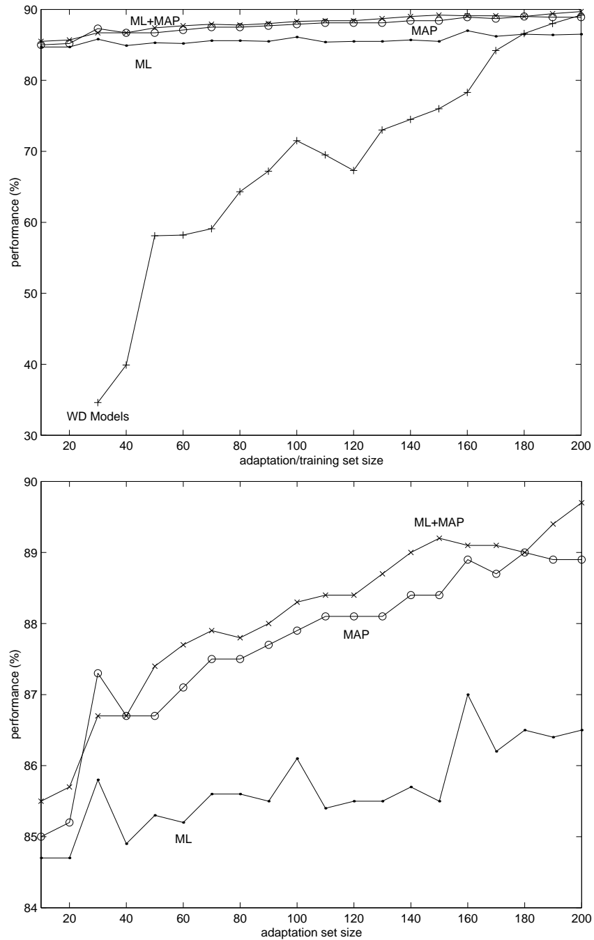
Figure 5: The upper figure reports the accuracy vs the training/adaptation set size for the WD models and the WI models adapted with ML, MAP and ML+MAP techniques. In the lower plot, the curves of the adapted models are shown in more details. The values are reported for training/adaptation set sizes less than or equal to 200. When the training/adaptation set size is less than 30, no WD system can be trained.
