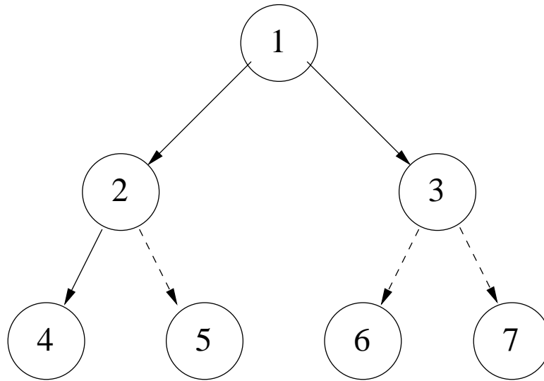
Figure 1: Regression tree with four base classes. The dashed line means that the child node does not contain sufficient data. In the case of the figure, there are three regression classes. The first one is composed of data clustered at node 4. They are transformed by a matrix estimated with the data themselves. The second one is composed of data clustered at node 5. Their transform matrix is estimated using data clustered at node 2 because the data belonging to node 5 are not enough. The last class is composed of data clustered at nodes 6 and 7. Since the data are insufficient for both nodes, they share a common transform matrix estimated with the data clustered at node 3 and then form a single class.
