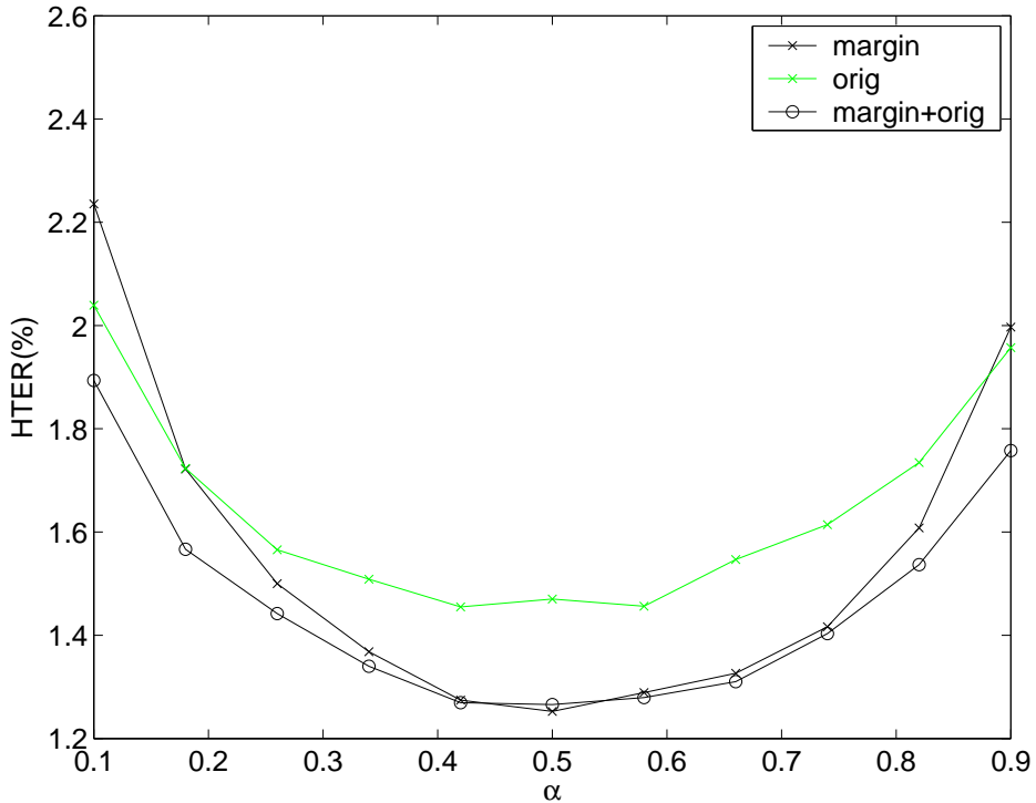
Figure 2: Pooled EPC curves of fusion experiments using original expert opinion (labeled as “orig”), product of expert opinion with margin (labeled as “margin”), and combination of both information (labeled as “margin+orig”), all using the mean operator. According to the HTER significant test, the “margin+orig” curve is always better than the “orig” curve, at different \alpha , at 95% of confidence. These experiments were carried out on the XM2VTS database using 32 intramodal and multimodal fusion datasets, and each dataset contains the scores of two experts.
