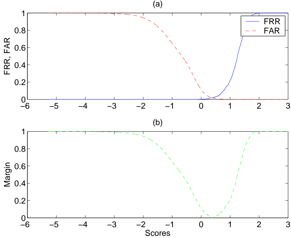
Figure 1: (a) FAR and FRR as a function of the threshold in the score space. (b) The derived margin based on (a).
