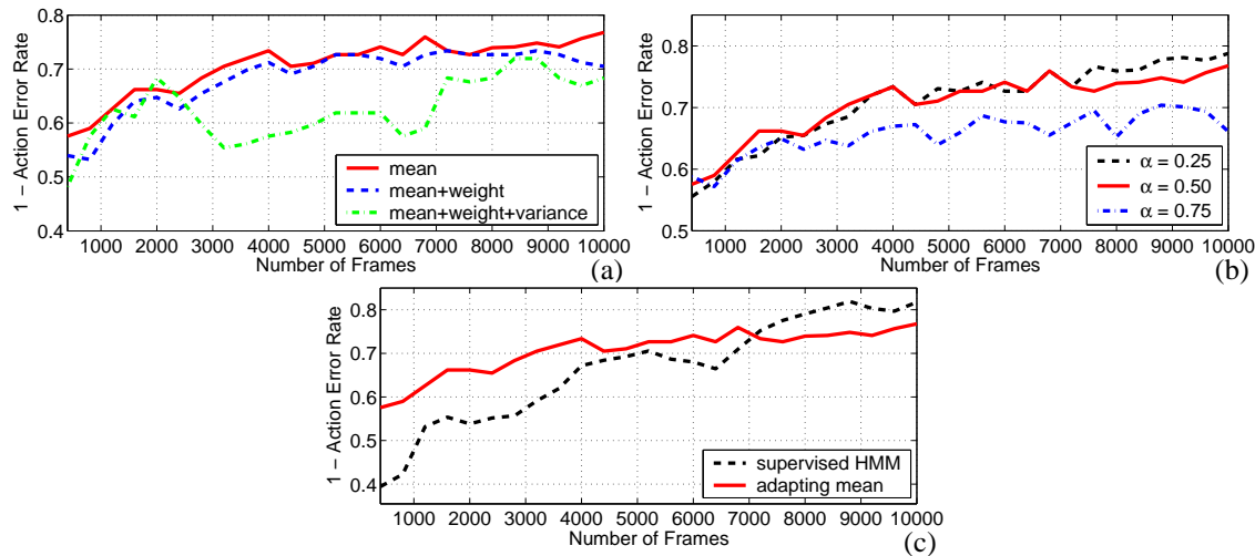
Figure 2: (a) Results of the semi-supervised method for adapting different parameter combinations. (b) Results of the semi-supervised method for different \alpha values. (c) Comparison of the semi-supervised and the supervised methods. The x-axis represents the number of labeled frames used in model training / adaptation (features were extracted at 5 frames per second).
